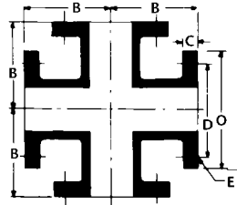
Cross - Flanged
